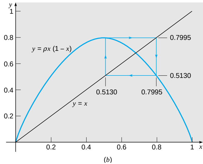
FIGURE 2.9.4 A solution of u_{n+1} = \rho u_n(1 - u_n) for \rho = 3.2 ; period two. (a) u_n versus n ; (b) a two-cycle.
